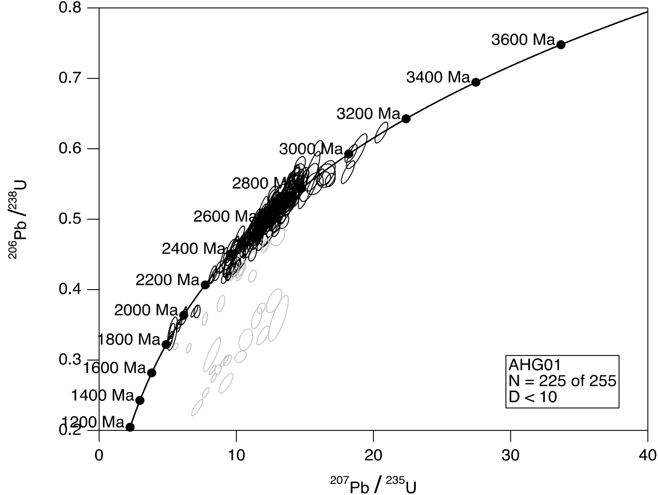
Concordia Diagram
