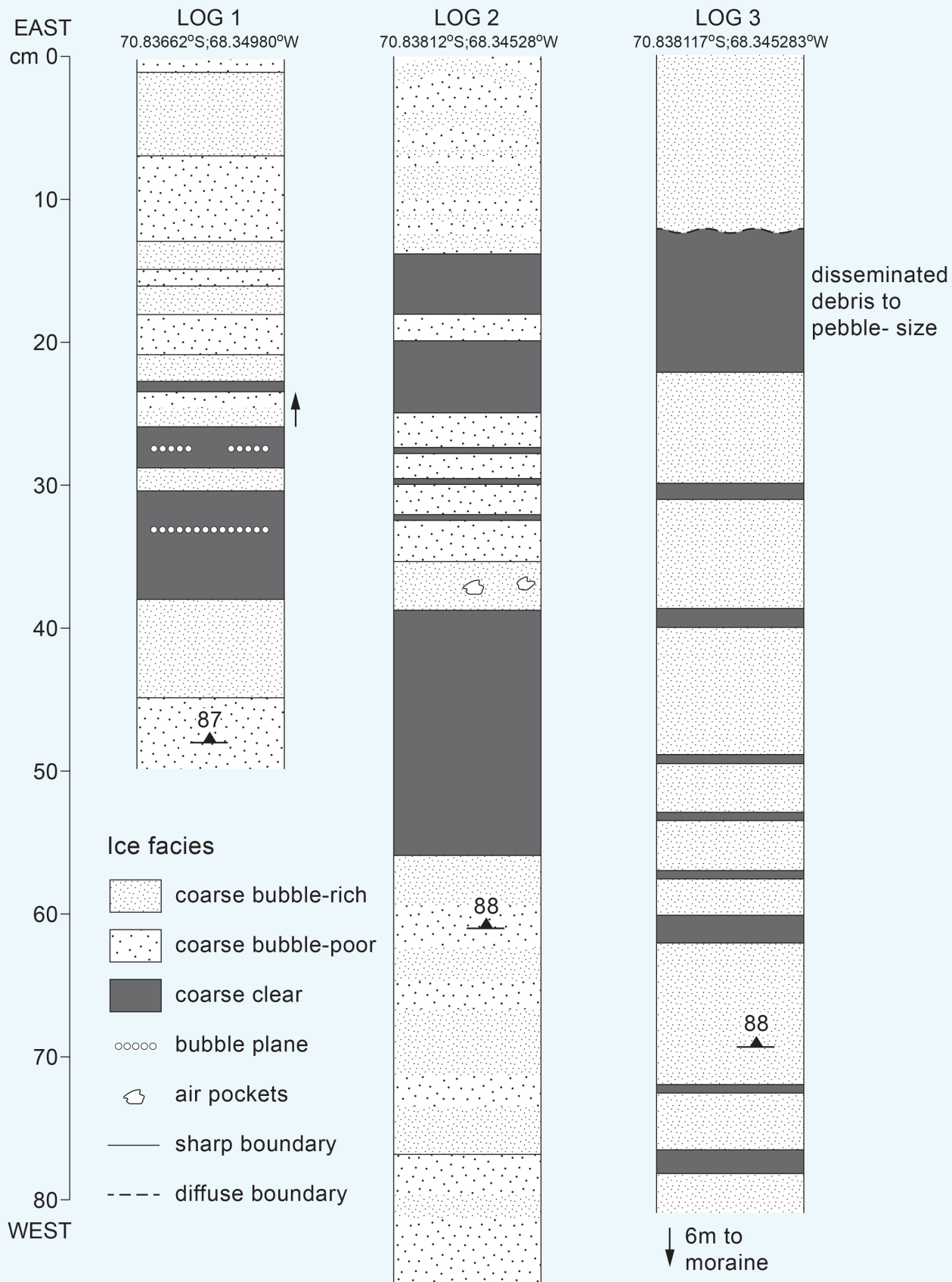
Logs of ice facies in foliation
